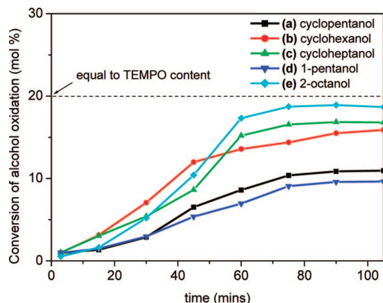
Figure 4. ^1\text{H} NMR monitoring the alcohol conversion in the reaction mixture: (a) cyclopentanol, (b) cyclohexanol, (c) cycloheptanol, (d) 1-pentanol, and (e) 2-octanol.
