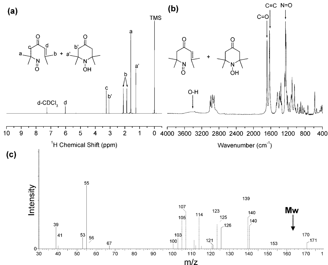
Figure 3. Structural identification of a mixture of N -hydroxy-4-oxo-2,2,6,6-tetramethylpiperidine and 2,6-dimethyl-6-nitrosohept-2-en-4-one using (a) ^1\text{H} NMR and (b) FTIR spectroscopy and (c) mass spectrometry.
