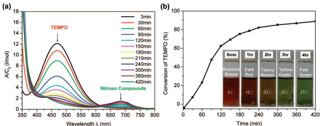
Figure 1. (a) UV-vis spectra and (b) TEMPO conversion of the reaction mixture containing BPO, TEMPO, and styrene at various time intervals during ambient warming from 0 to 25 °C (A: UV-vis absorbance; C_0 : initial concentration of TEMPO in solution; UV-vis quantification at 469.5 nm).
